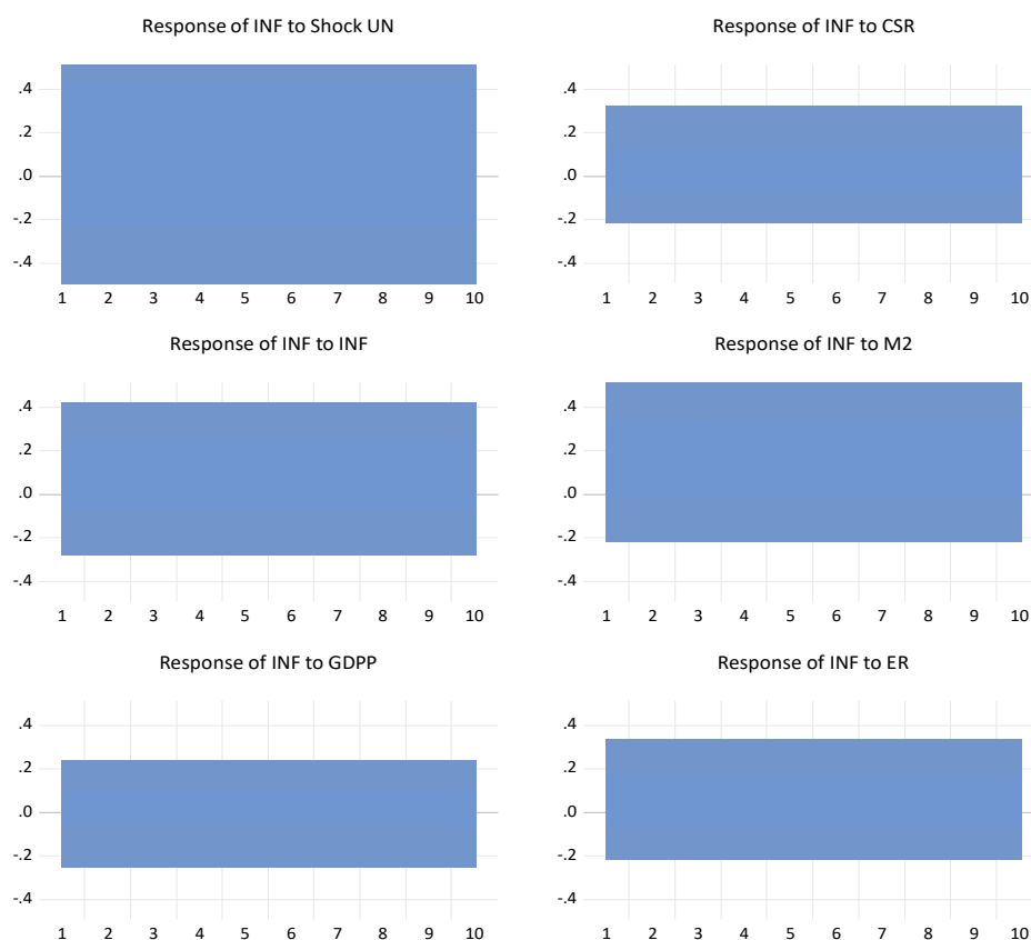
Response to Structural VAR Innovations 95% CI using analytic asymptotic S.E.s
